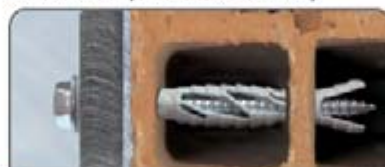
Behavior on perforated masonry
