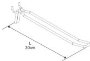
GNC 02 25 030 Special double hook length 30 cm
