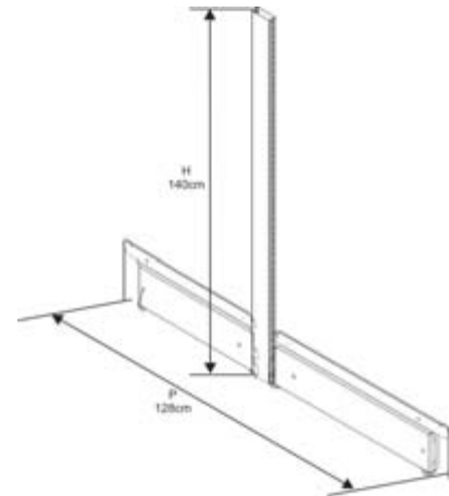
PNT 02 00 140 Uprights for "gondola" stand h 140 cm
