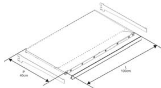
RPN 01 40 100 40 x 100 cm
