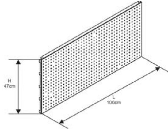
PAN 01 47 100 Perforated back panel
