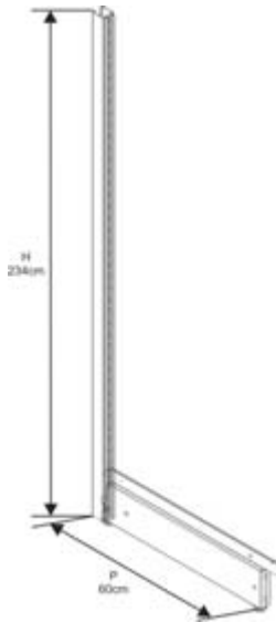
PNT 01 00 234 Uprights for wall stand h 234 cm
